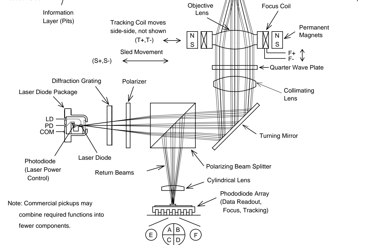
General Three-Beam Optical Pickup Organization
