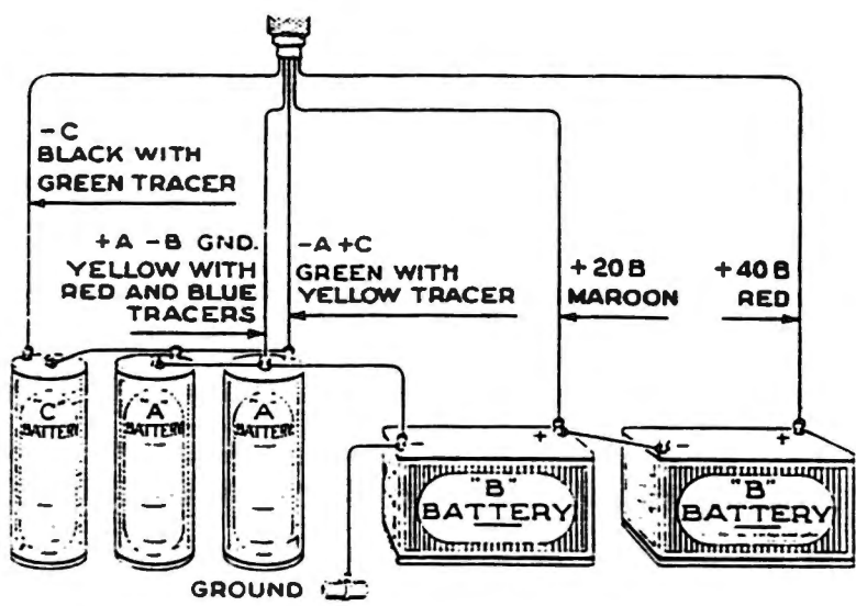
Fig. 2—Battery Connections
